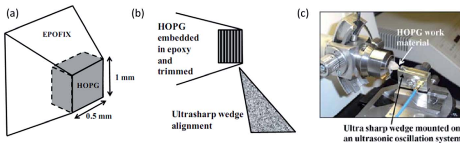
Fig. 3 (a) HOPG mounted in epofix and trimmed to a pyramid shape. (b) Setup showing the wedge alignment with HOPG layers. (c) Actual experimental setup. Reproduced with permission from ref. 47. Copyright 2011 Springer.
