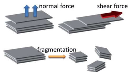
Fig. 1 Two kinds of mechanical routes for exfoliating graphite into graphene flakes and the auxiliary route for fragmentation.
